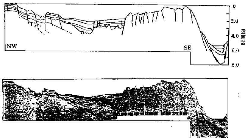
图6 横穿海槽南部反射地震剖面 Fig.6 Seismic profile of the southern Okinawa Trough
