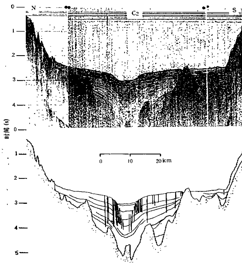
图7 横穿海槽中部的地震剖面(据 Herman, 1978) Fig.7 Seismic profile of the middle Okinawa Trough (By Herman, 1978)
